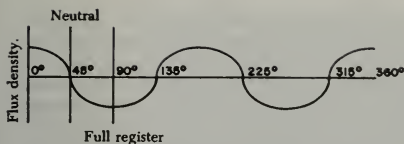
FIGURE 4-3. Change in flux density as magnet rotates.
